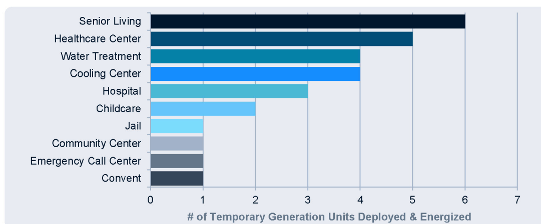
Figure 3 - 6: Temporary generation Units Deployed &amp; Energized
