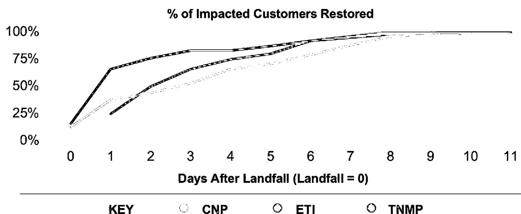
Figure 2 - 7: Beryl Restoration Curves of Peer Utilities 20
