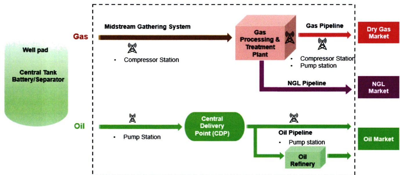
Figure 4-1: Production supply chain with power requirements
