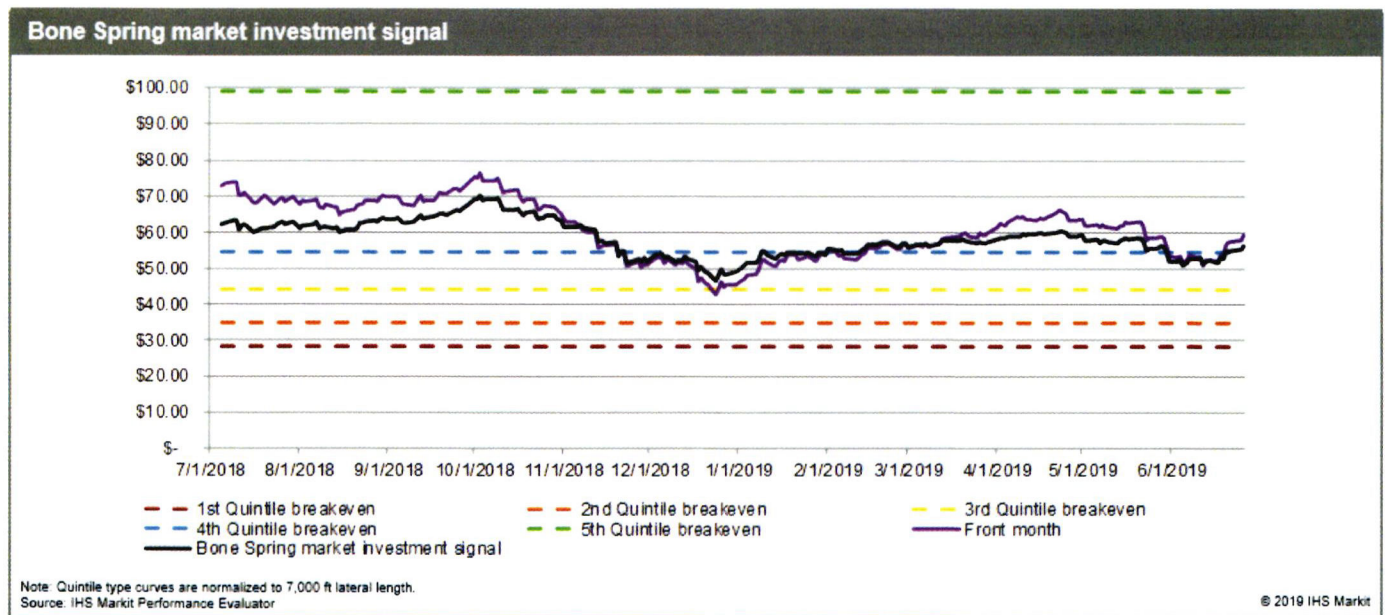
Figure 1-20. Bone Spring well economics by quintile
