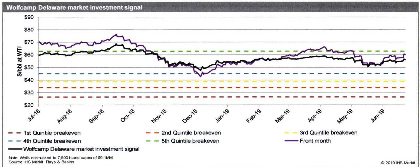
Figure 1-19. Wolfcamp Delaware well economics by quintile
