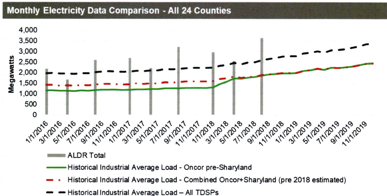
Figure 3-6: Monthly electricity data comparison – all counties
