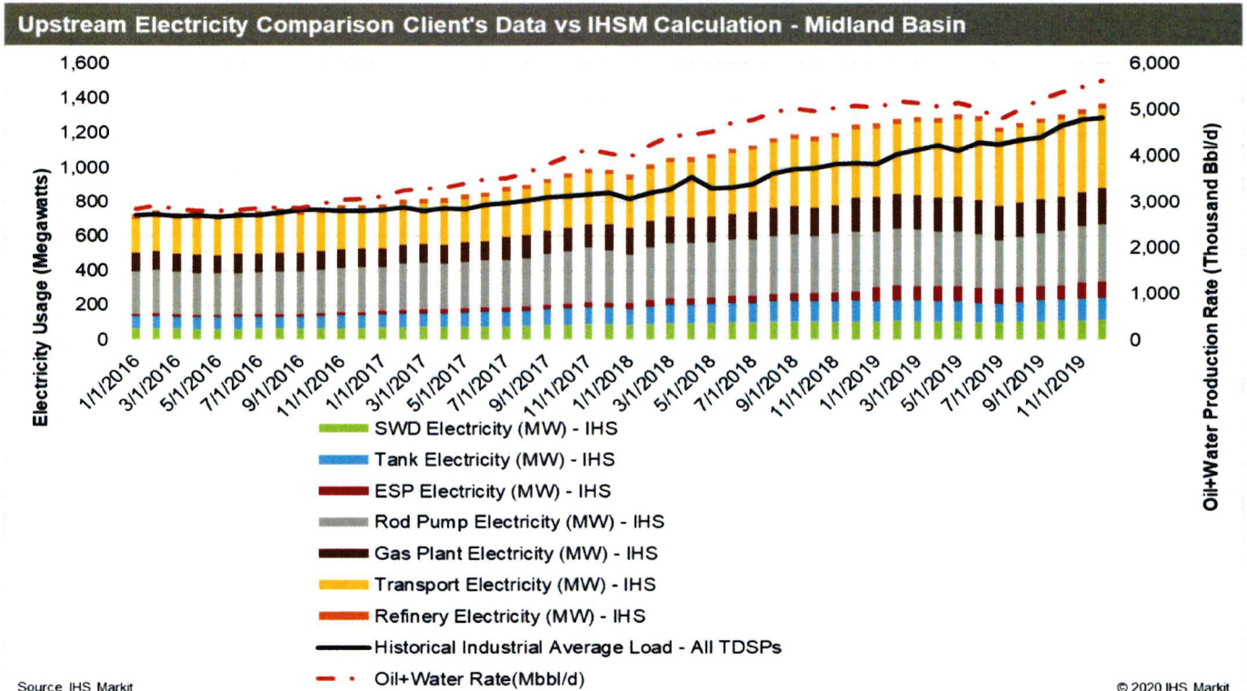
Figure 4-6 Midland Basin upstream electricity usage comparison
