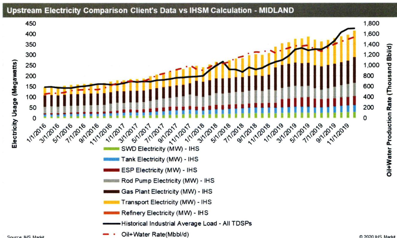
Figure 4-1. Upstream electricity comparison
