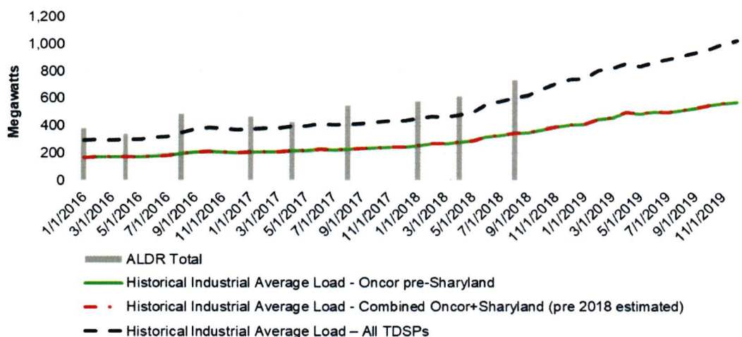
Figure 3-3: Monthly electricity data comparison for the Delaware Basin
