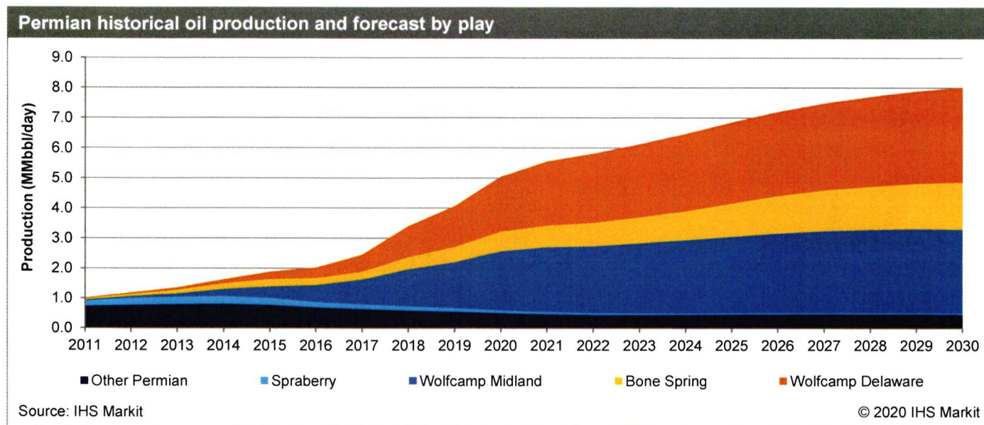
Figure 1-5. IHS Markit forecast for Permian Basin production, by play
