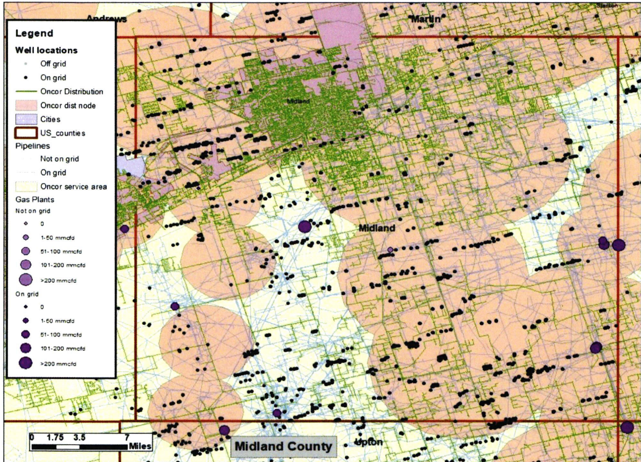
Figure 4-3. Midland county map showing oil and gas activity and electrical transmission
