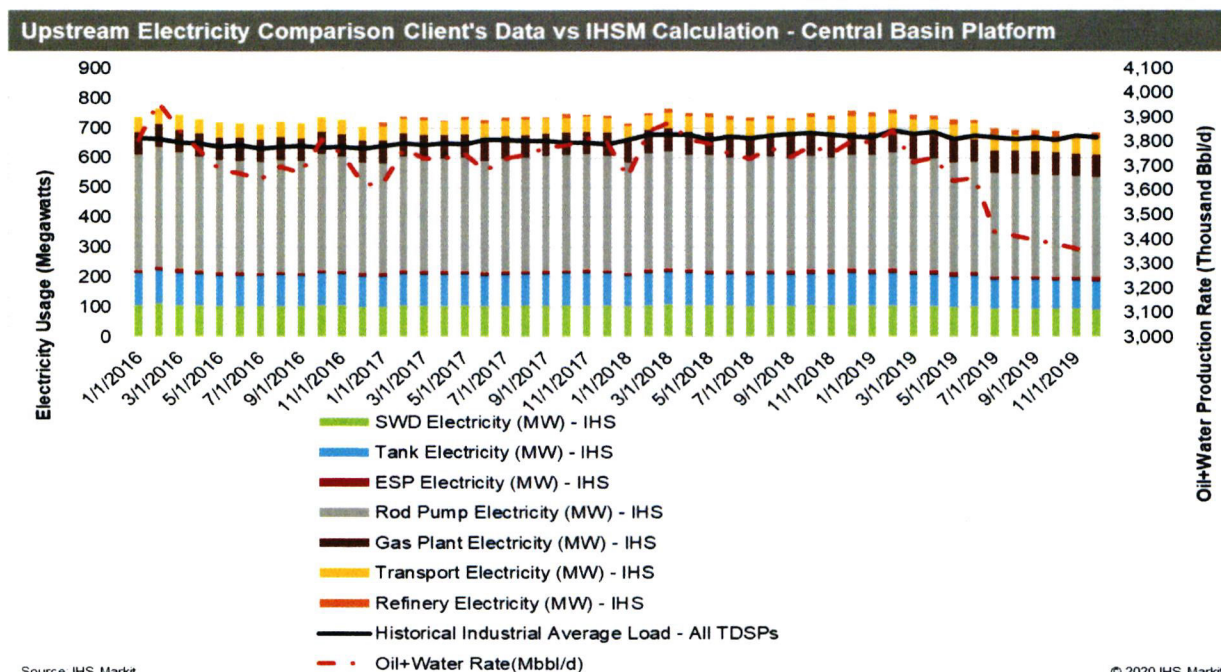
Figure 4-4. Central Basin Platform upstream electricity comparison
