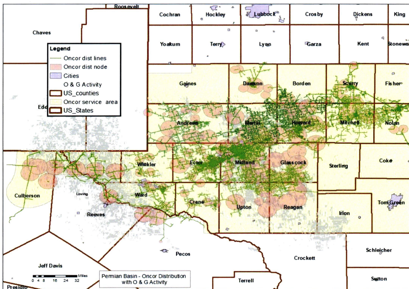
Figure 4-2. Regional electric distribution map
