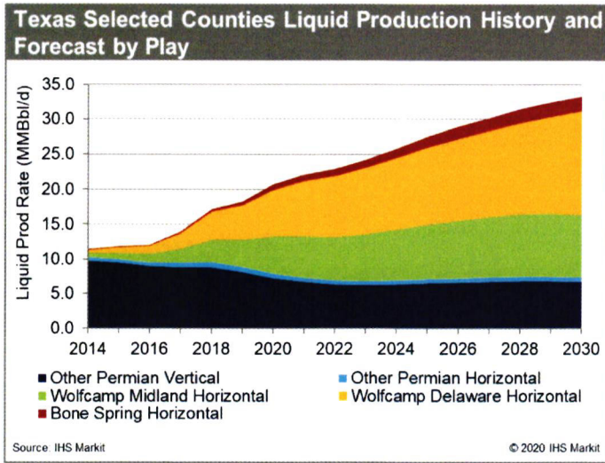
Figure 2-5: Texas Selected Counties Liquid Production History and Forecast by Play
