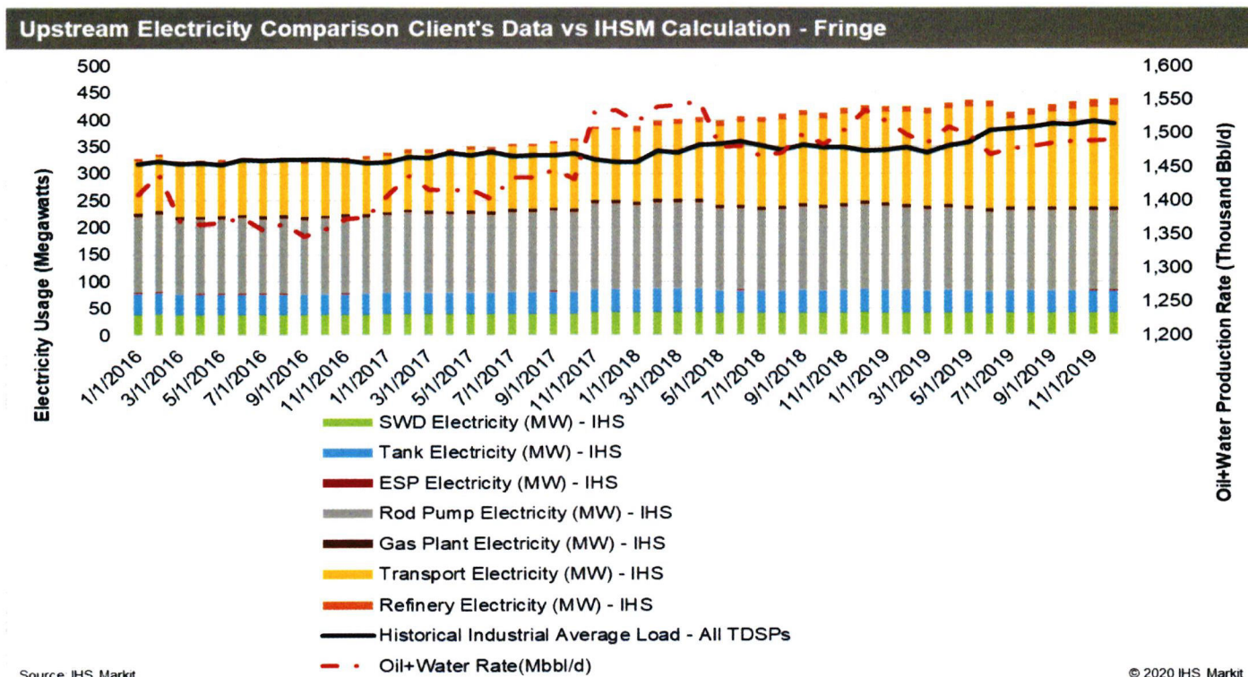
Figure 4-7. Fringe upstream electricity usage comparison
