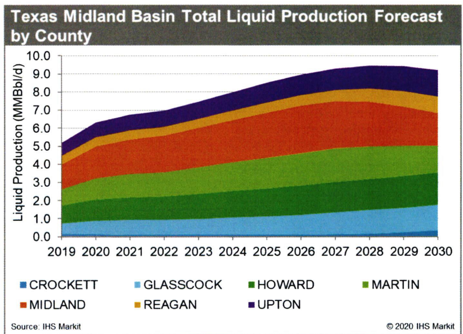
Figure 2-15: Texas Midland Basin Region Total Liquid Production by County
