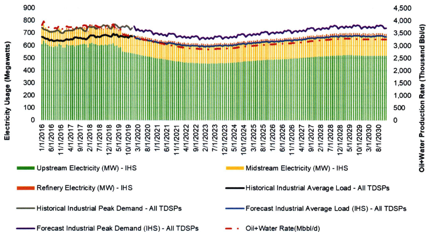
Figure 5-8. Industrial electricity forecast – Central Basin Platform
