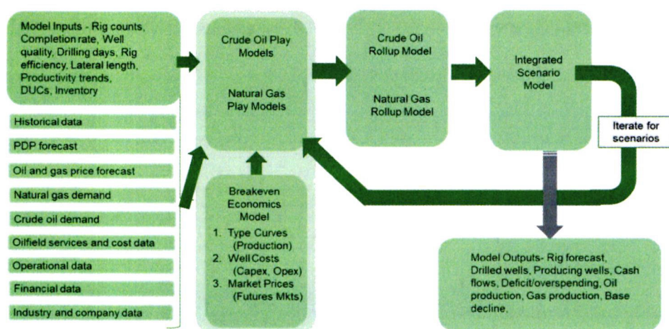
Figure 1-4. IHS Markit production forecast workflow chart
