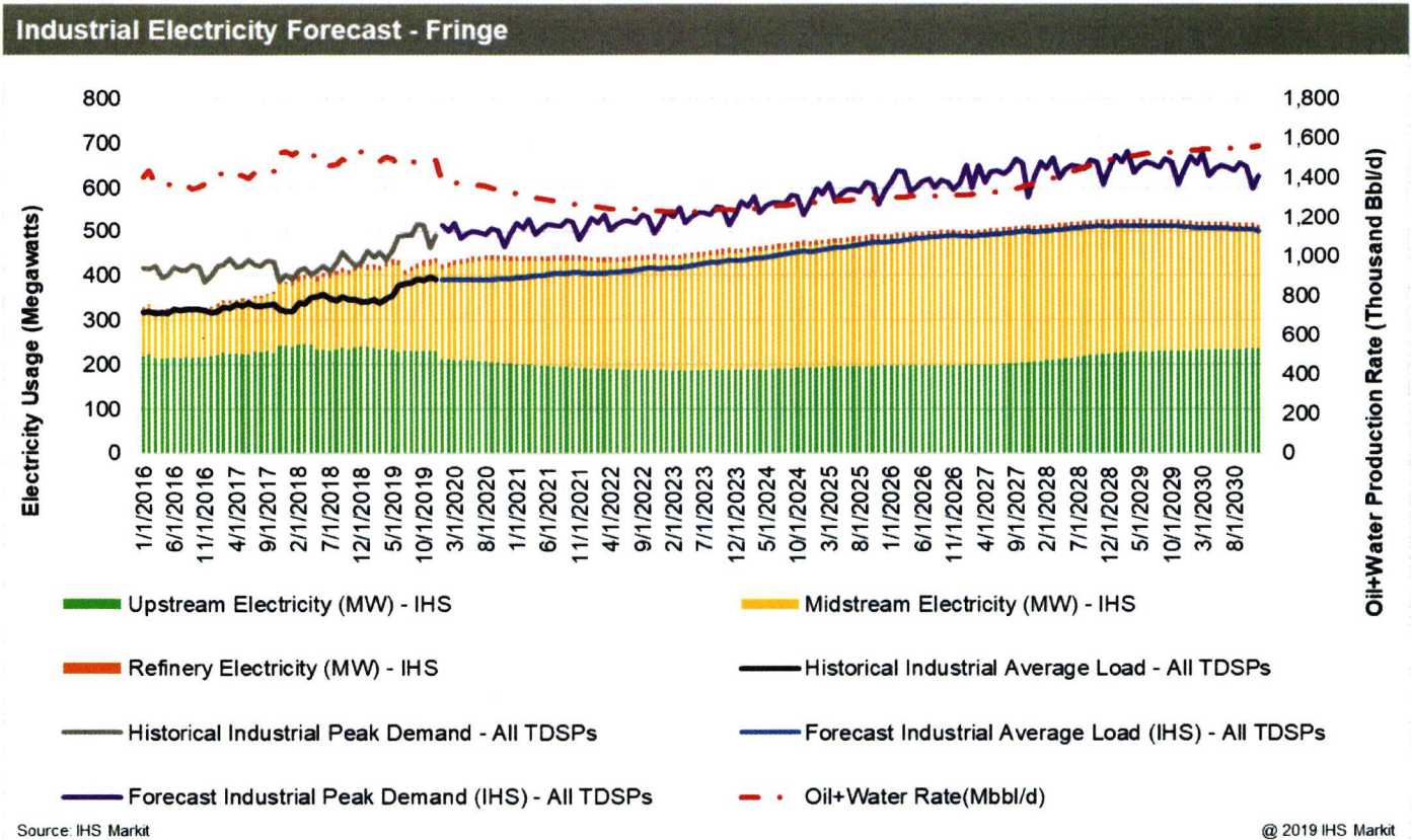
Figure 5-9. Industrial electricity forecast – Fringe counties
