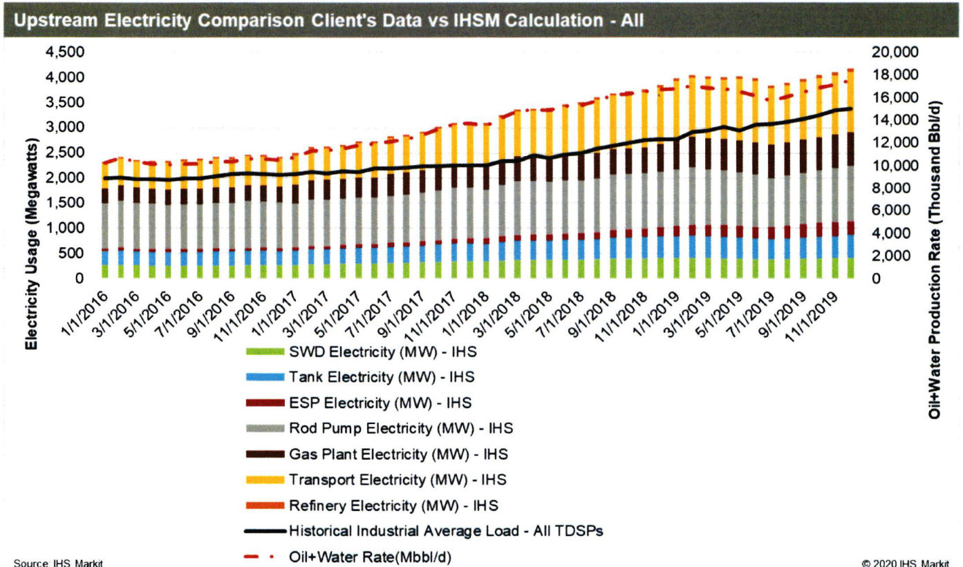
Figure 4-8. Summary of the upstream usage from oil and gas activities and Oncor billing data history
