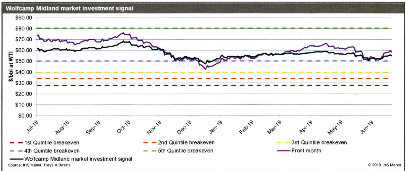
Figure 1-18. Wolfcamp Midland well economics by quintile
