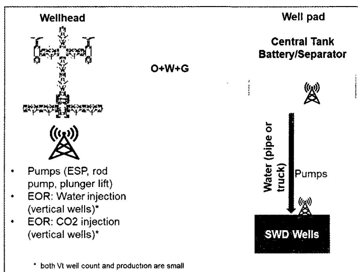
Figure 3-1 Upstream Schematic
