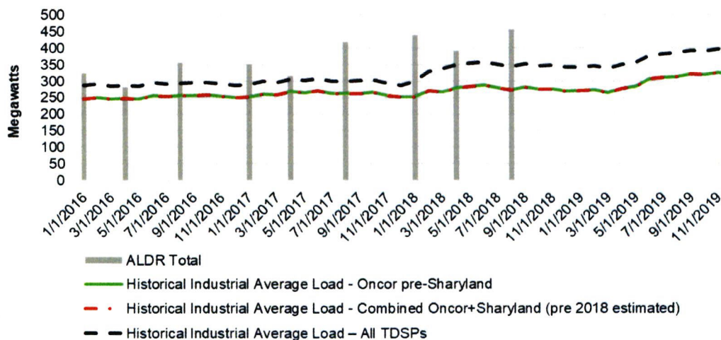
Figure 3-5: Monthly electricity data comparison for the Fringe area
