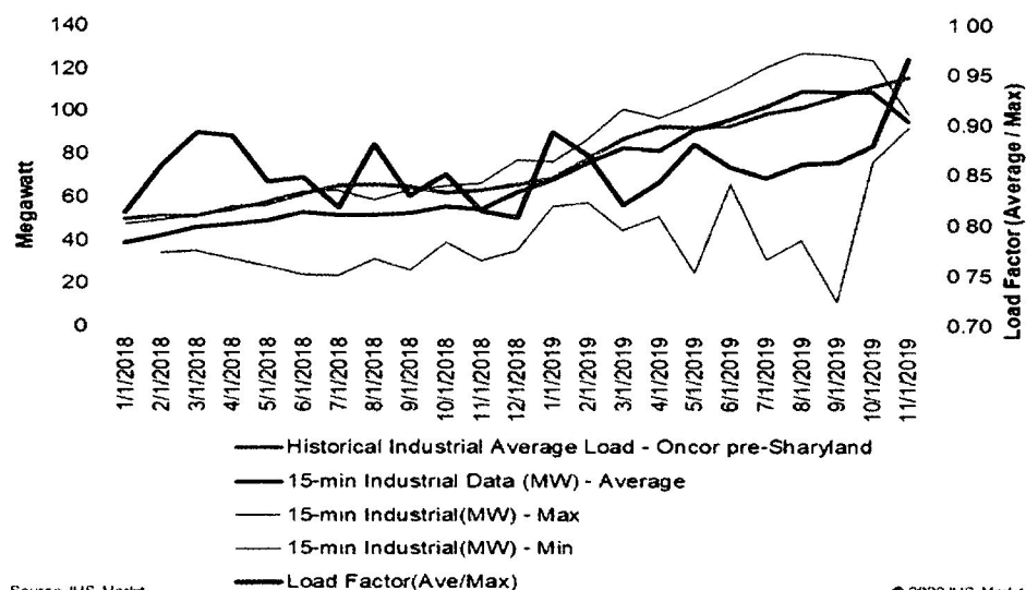
Figure 2.4: Loving and Midland County Basin 15-Minute Interval Data
