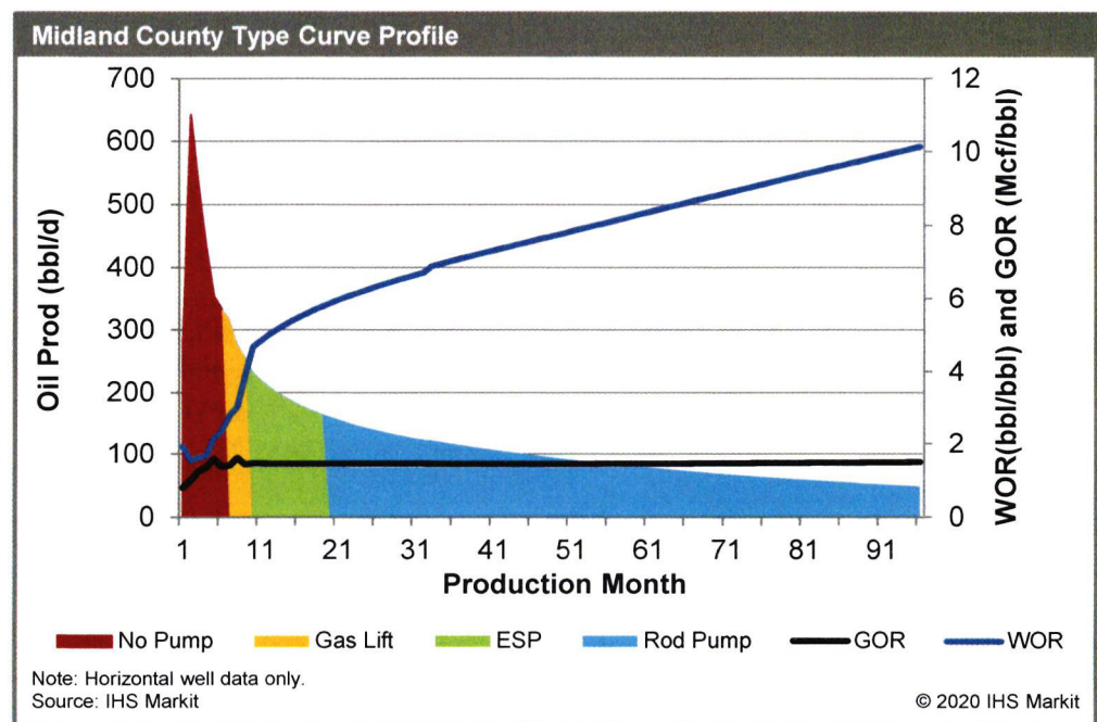
Figure 3-4 Example Type Curve -- Midland County
