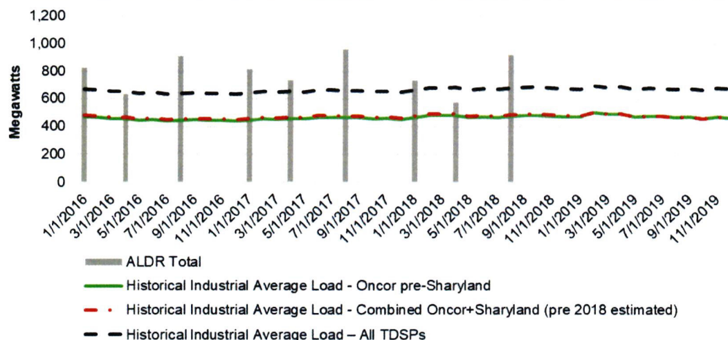
Figure 3-2: Monthly electricity data comparison for Central Basin Platform
