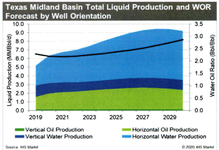
Figure 2-14: Texas Midland Basin Total Liquid Production and WOR Forecast
