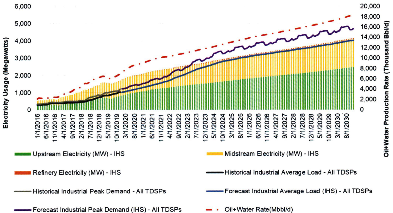
Figure 5-6. Industrial electricity forecast – Delaware basin
