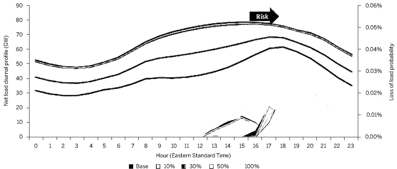
FIGURE 6 Shifting Periods of Risk in MISO with Increasing Levels of Solar Photovoltaics
