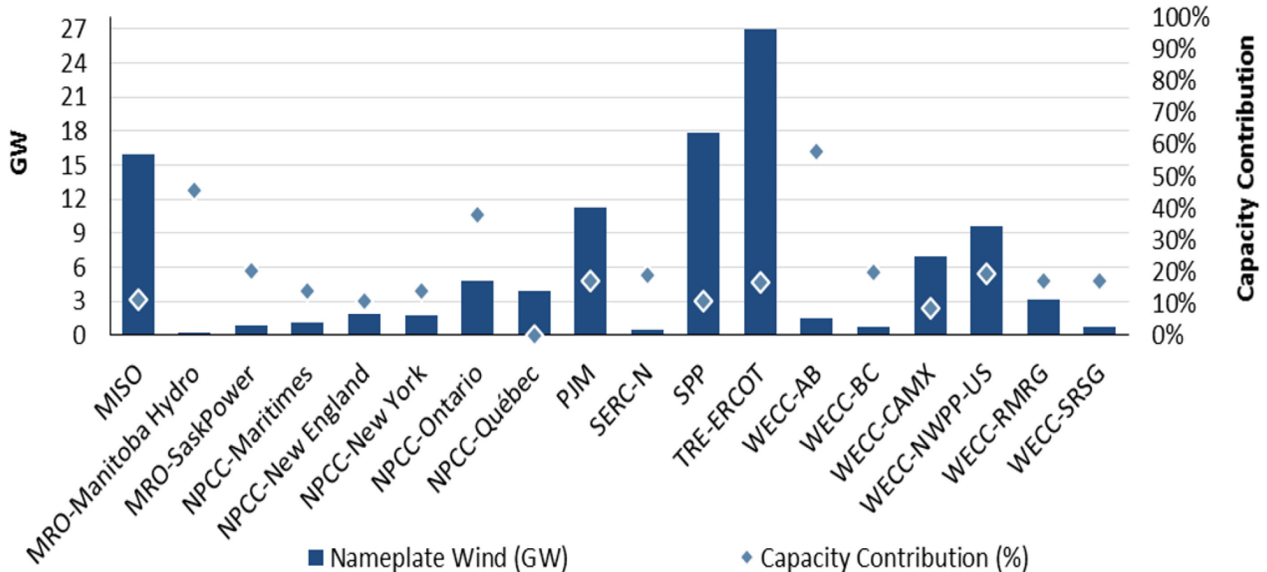
Figure 2.3: 2026 Existing and Tier 1 Wind
