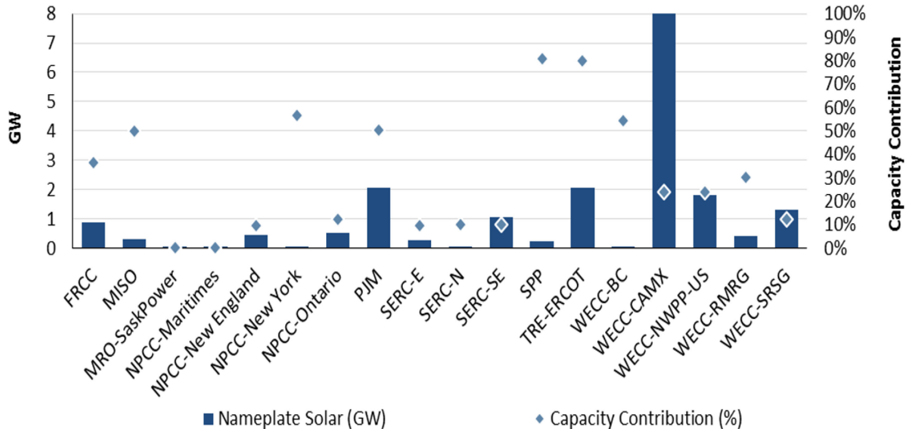
Figure 2.4: 2026 Existing and Tier 1 Solar
