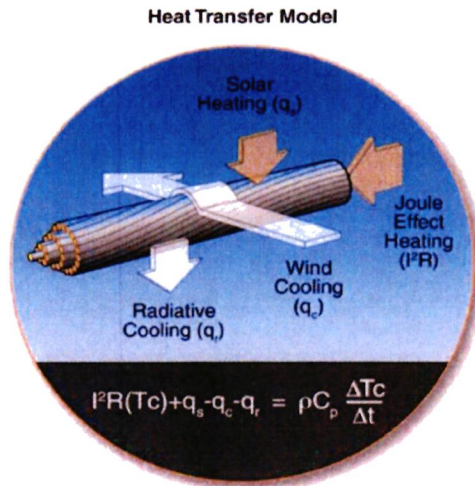
Figure 1: Heat-transfer model for a conductor.
