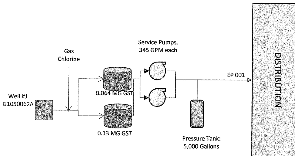
Schematic of City of Mountain City Water System
