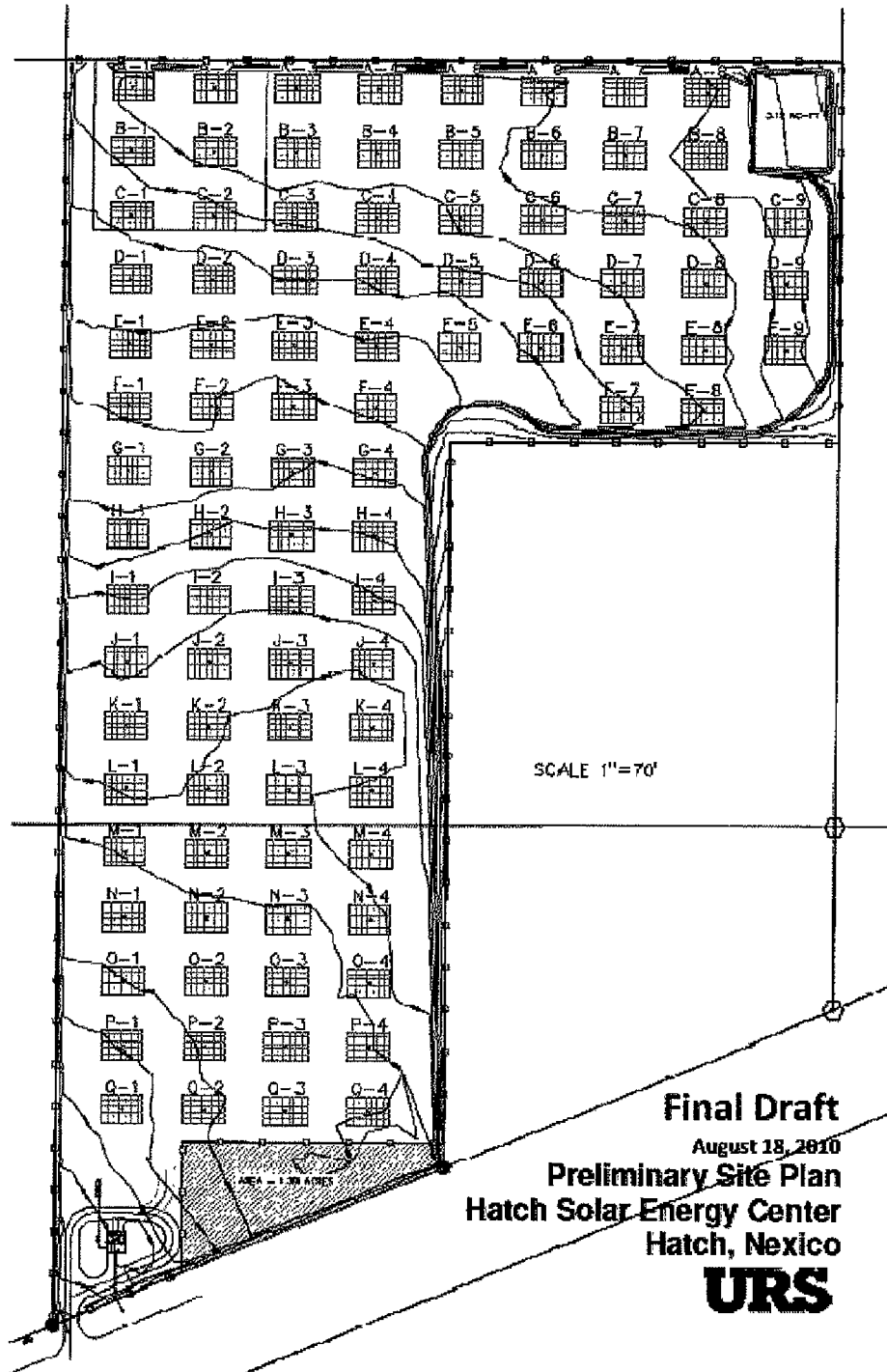
Preliminary Site Layout
