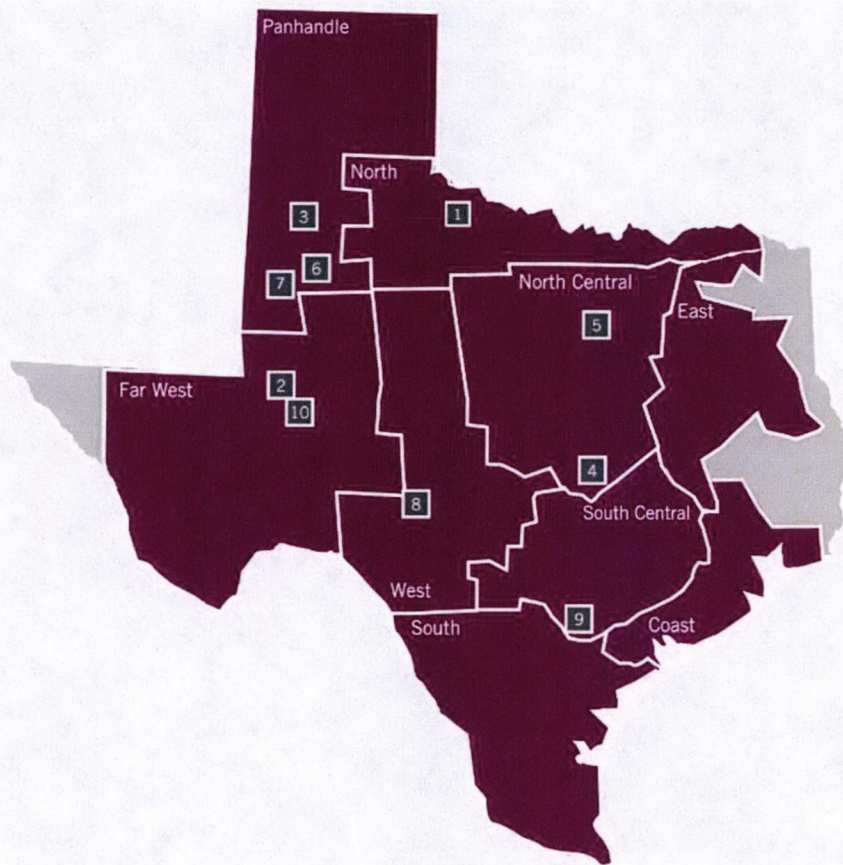
Figure ES.3: Transmission Additions Identified for Current Trends Scenario
