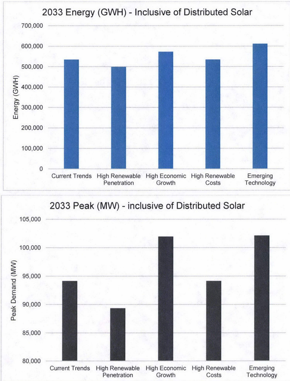
Figure I. 7: Energy and Peak for 2033 across the Five Scenarios
