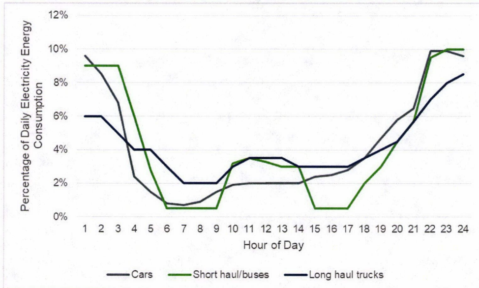
Figure 9: Assumed Hourly Charging Patterns by Vehicle Type
