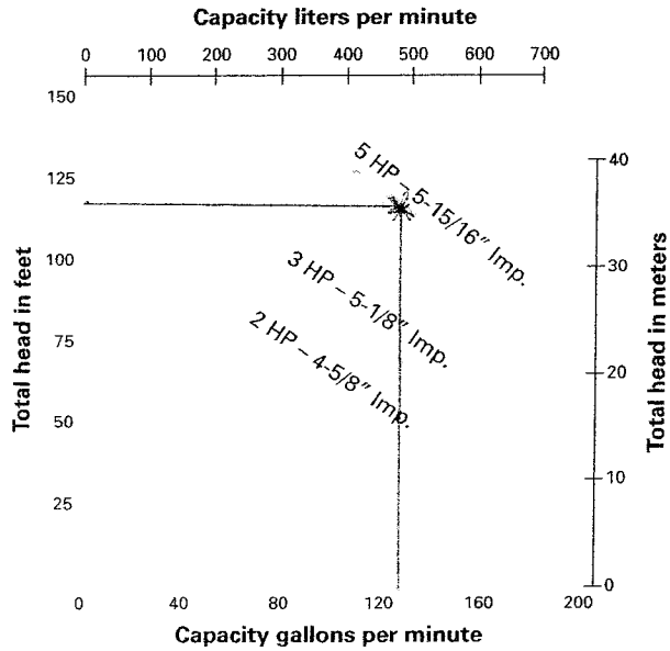
PUMP PERFORMANCE - 150M
