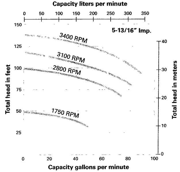
PUMP PERFORMANCE - 125B
