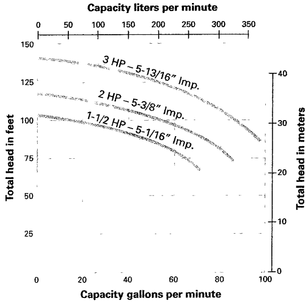
PUMP PERFORMANCE - 125M
