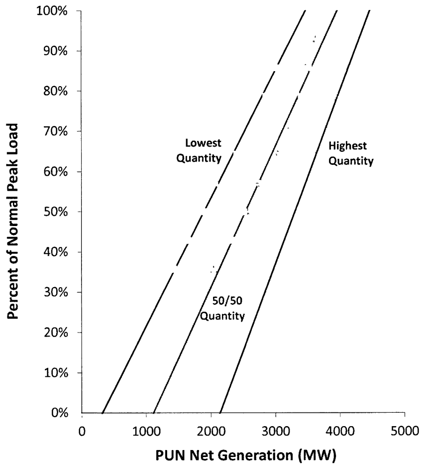
Figure A1-3 PUN Net Generation
