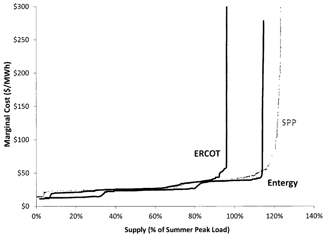
Figure A1-10 2022 System Supply Curves
