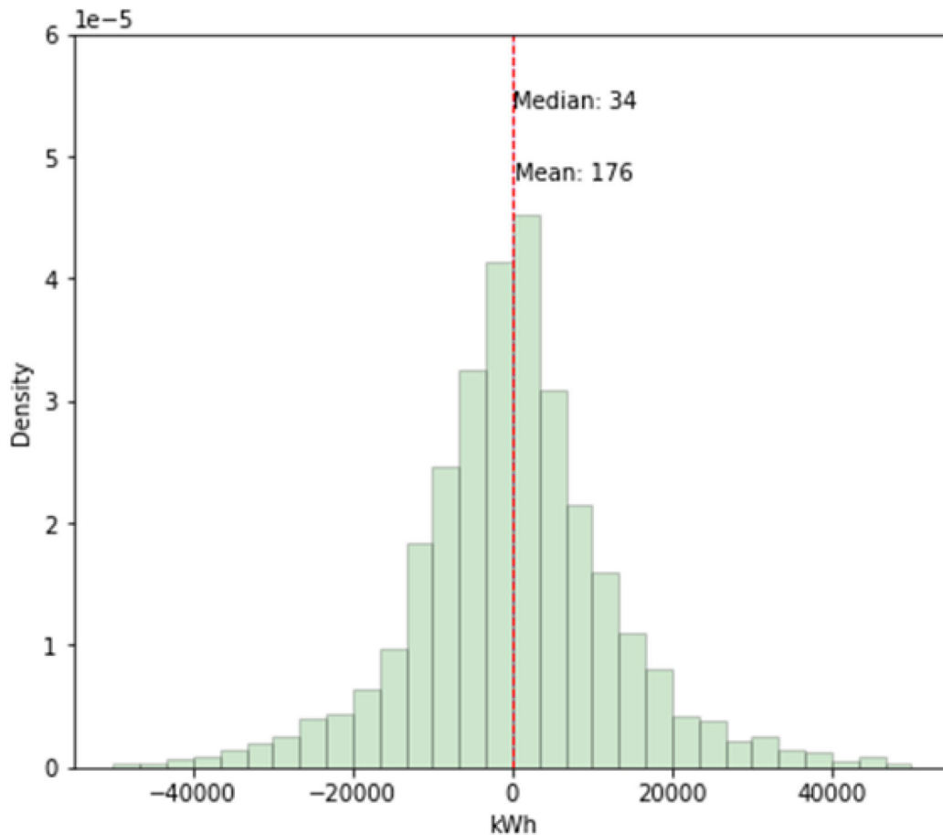
Figure 27. Weather-Normalized Air Infiltration kWh Consumption Before and After Installation
