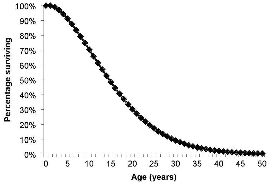
Figure 2. Central and Mini-Split AC/HPs—HP Survival Function 180
