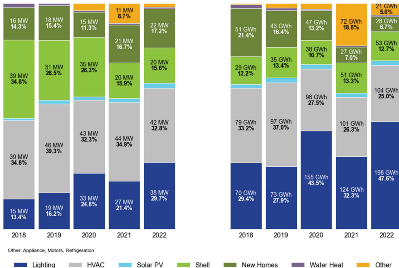
Figure 25. Distribution of Statewide Demand Reduction and Energy Savings by Measure Category—Residential Programs PY2018–PY2022 20
