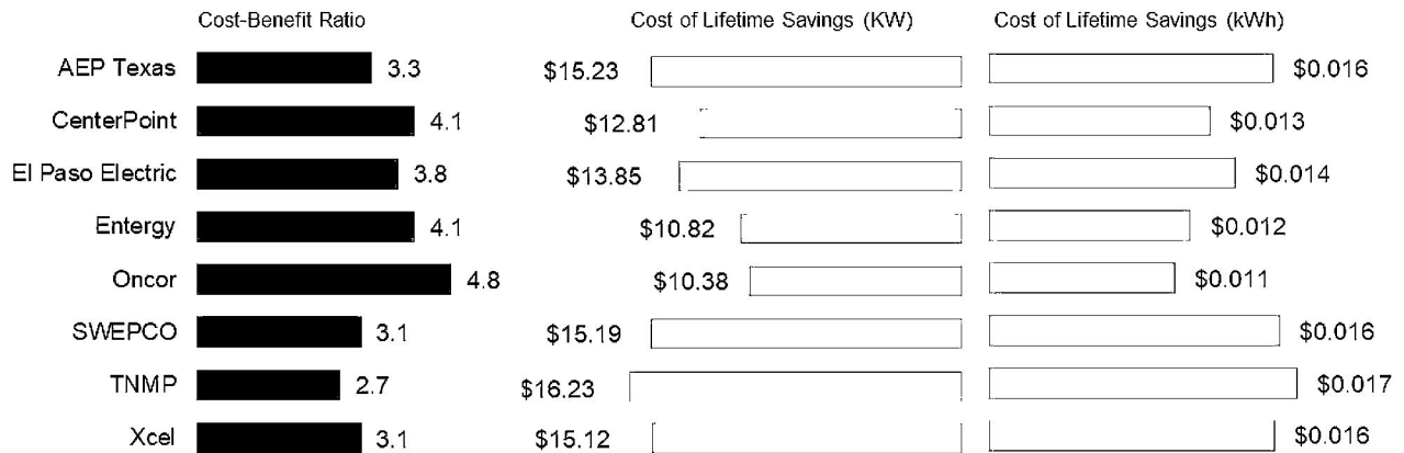
Figure 10. PY2022 Savings Cost-Benefit Ratio and Cost of Lifetime Savings
