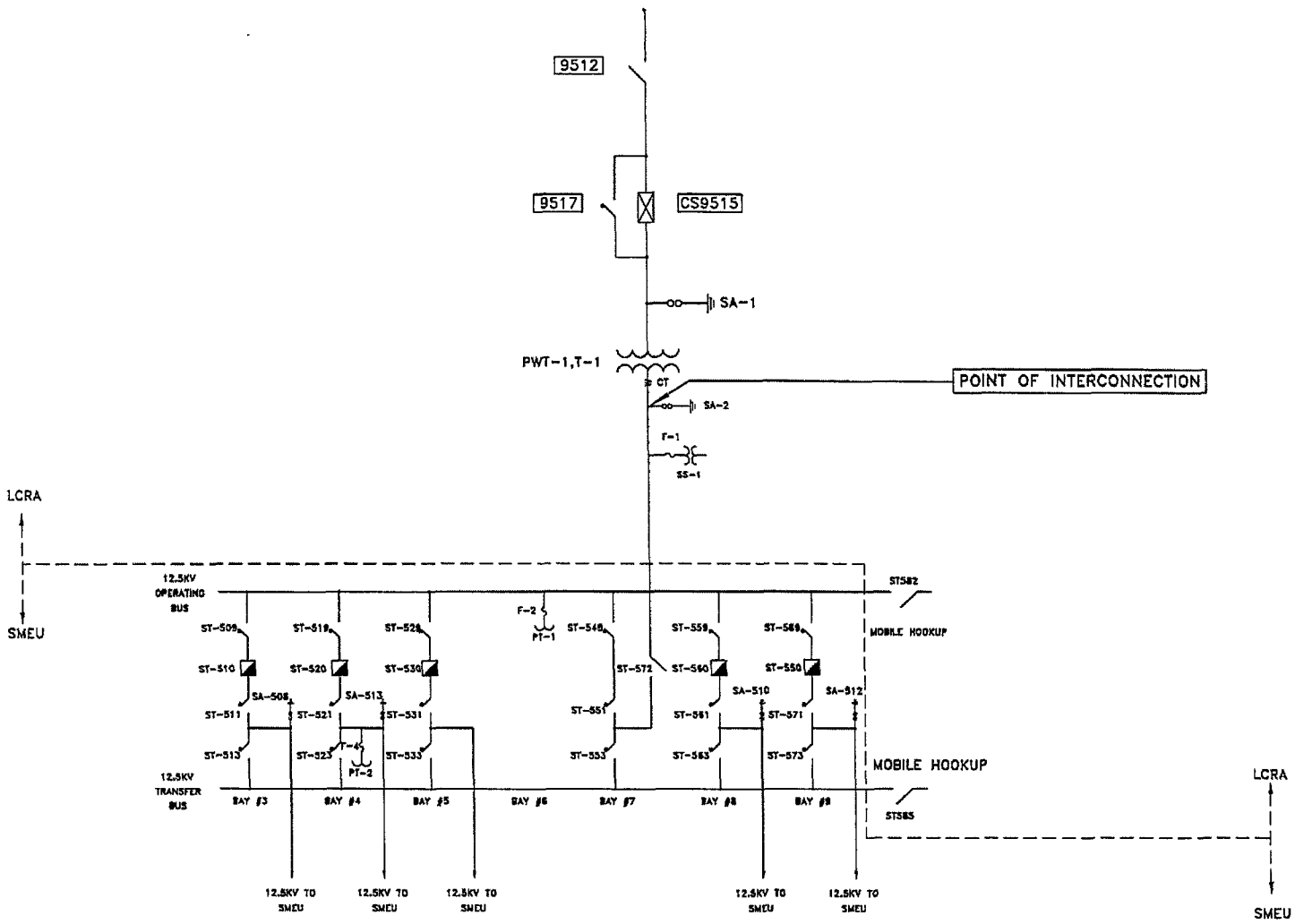
STRAHAN SUBSTATION
