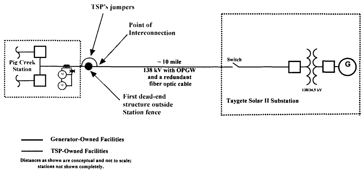
Conceptual One-Line Drawing of Point of Interconnection
