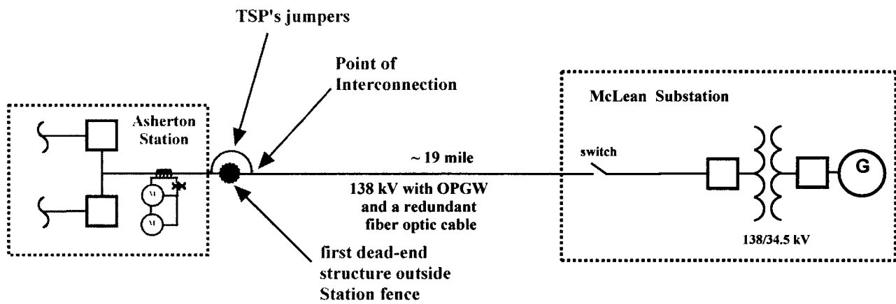
Conceptual One-Line Drawing of Point of Interconnection
