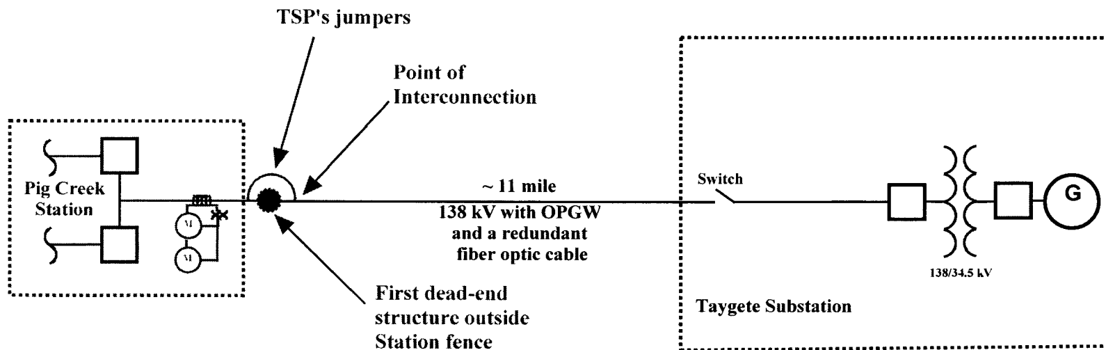
Conceptual One-Line Drawing of Point of Interconnection
