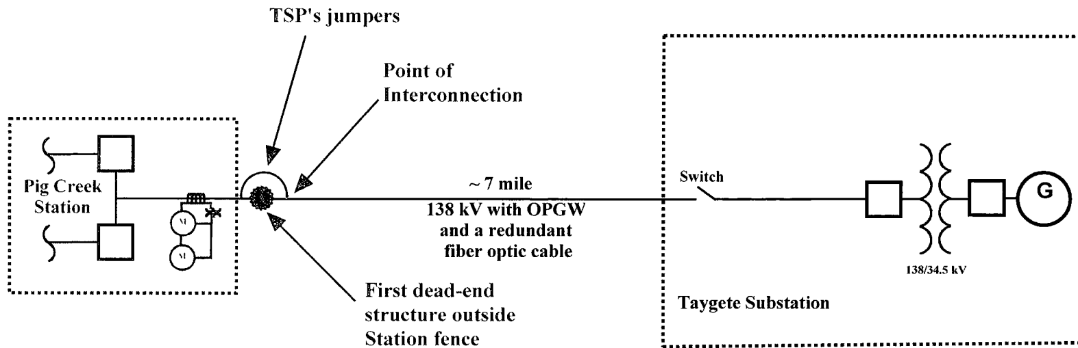
Conceptual One-Line Drawing of Point of Interconnection
