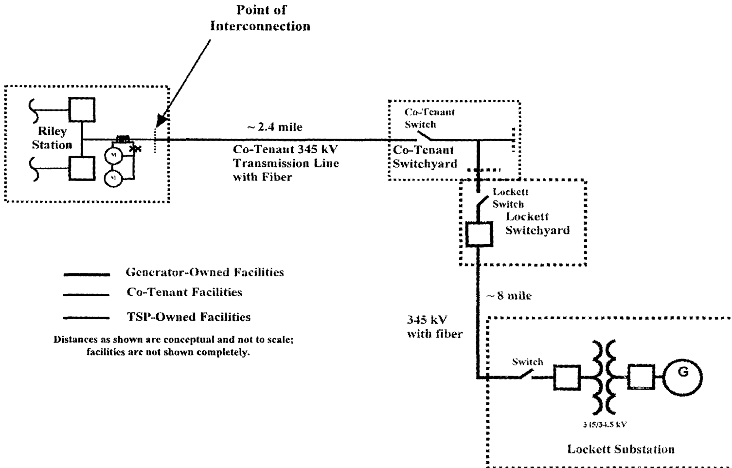
Conceptual One-Line Drawing of Point of Interconnection
