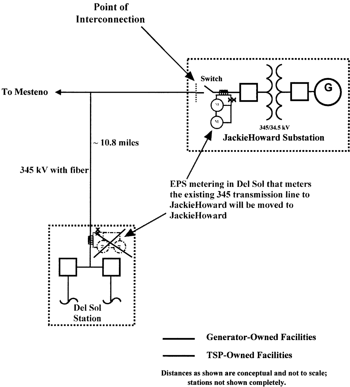
Conceptual One-Line Drawing of Point of Interconnection
