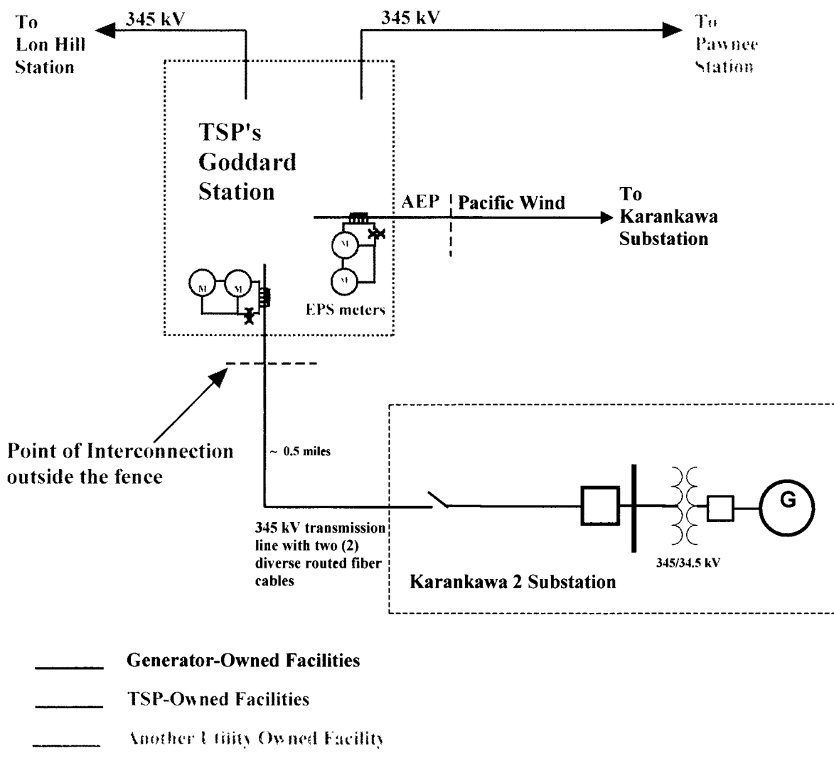
Conceptual One-Line Drawing of Point of Interconnection
