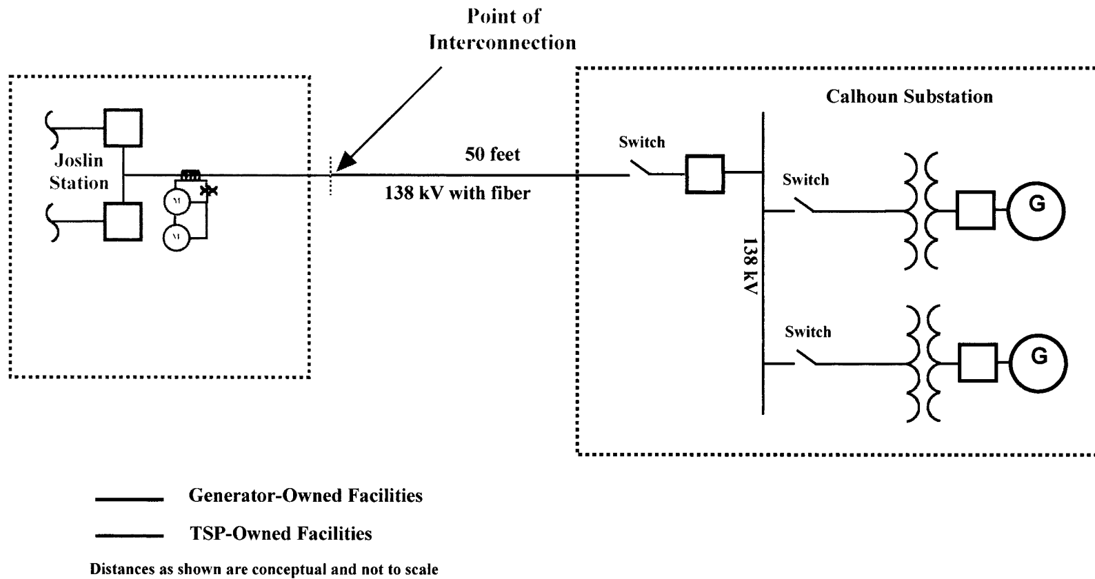
Conceptual One-Line Drawing of Point of Interconnection
