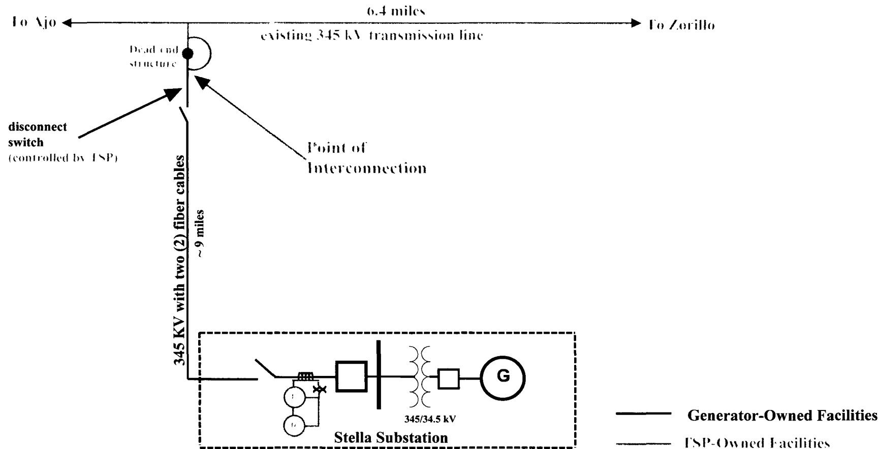
Conceptual One-Line Drawing of Temporary Facilities/Temporary Point of Interconnection
