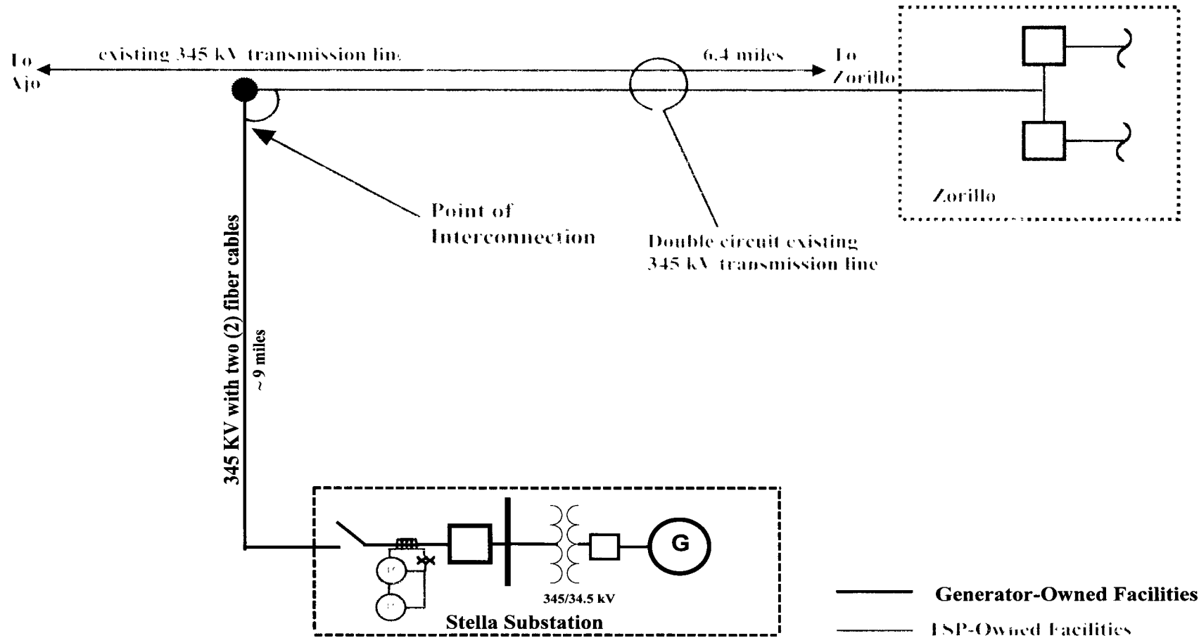
Conceptual One-Line Drawing of Permanent Facilities/Permanent Point of Interconnection
