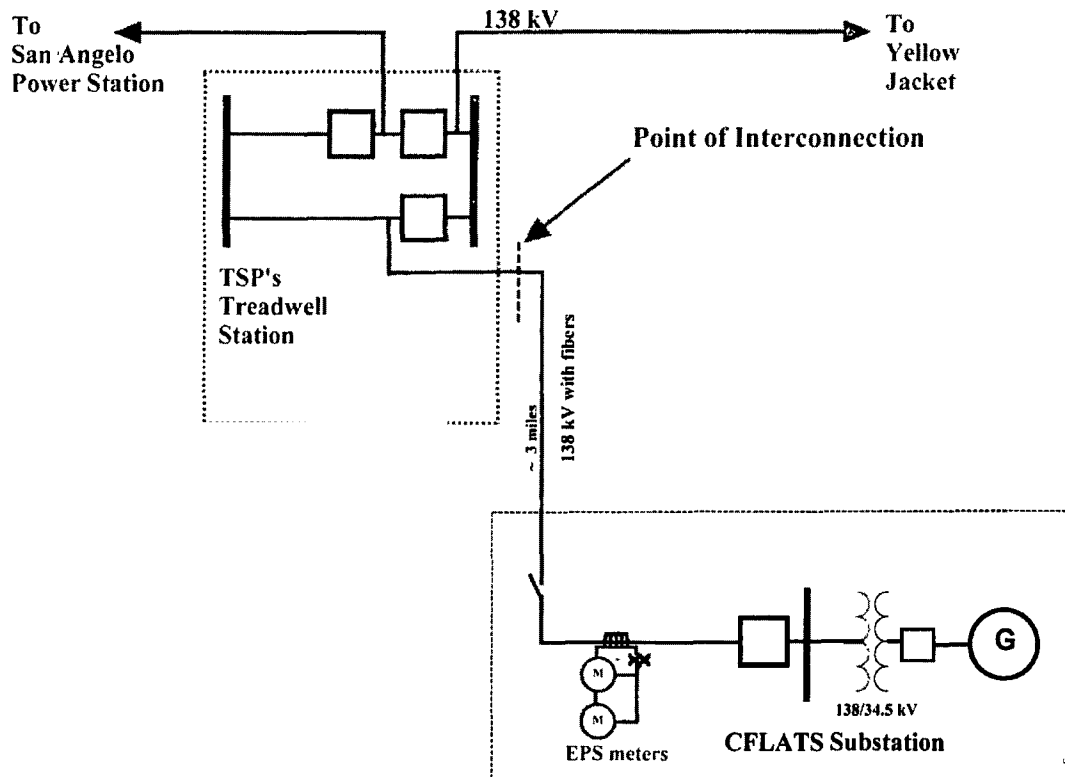
Conceptual One-Line Drawing of Permanent Facilities/Permanent Point of Interconnection
