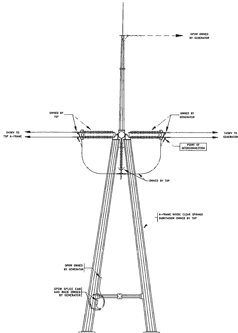
POINT OF INTERCONNECTION DETAIL #1
