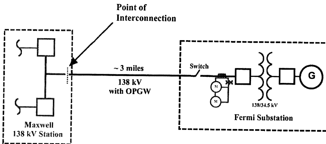
Conceptual One-Line Drawing of Permanent Facilities/Permanent Point of Interconnection
