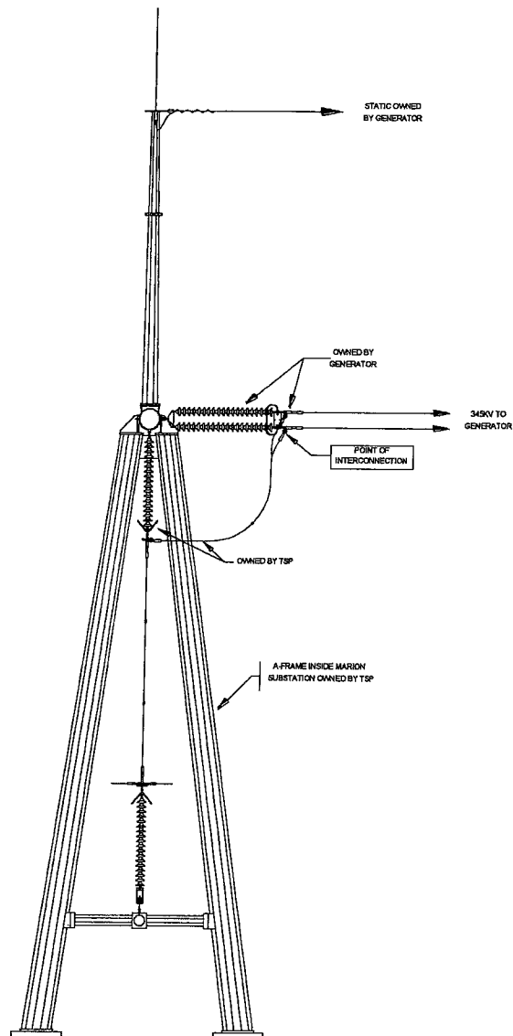
POINT OF INTERCONNECTION DETAIL #1
