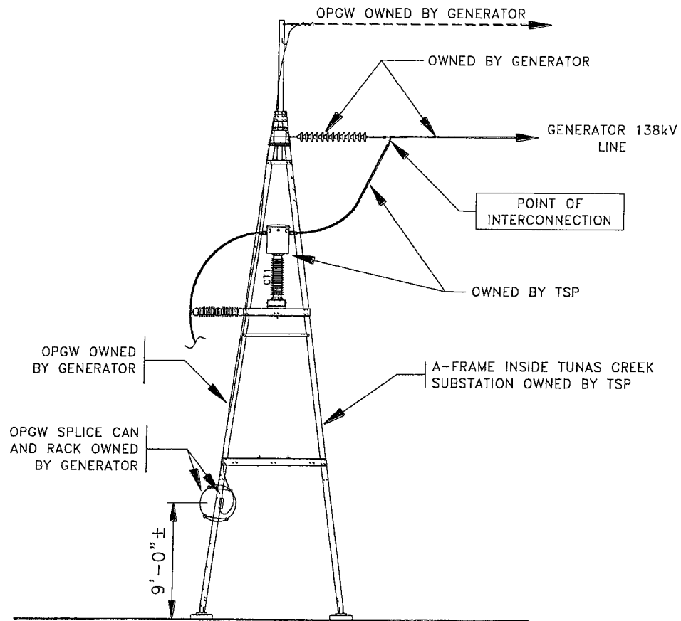
POINT OF INTERCONNECTION DETAIL
