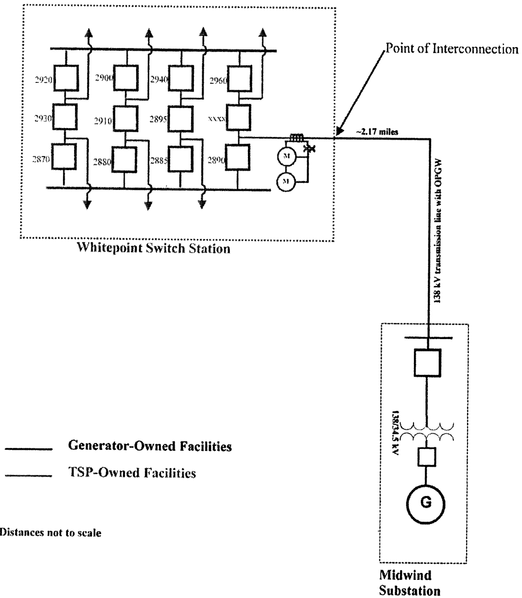
Conceptual One-Line Drawing of Point of Interconnection
