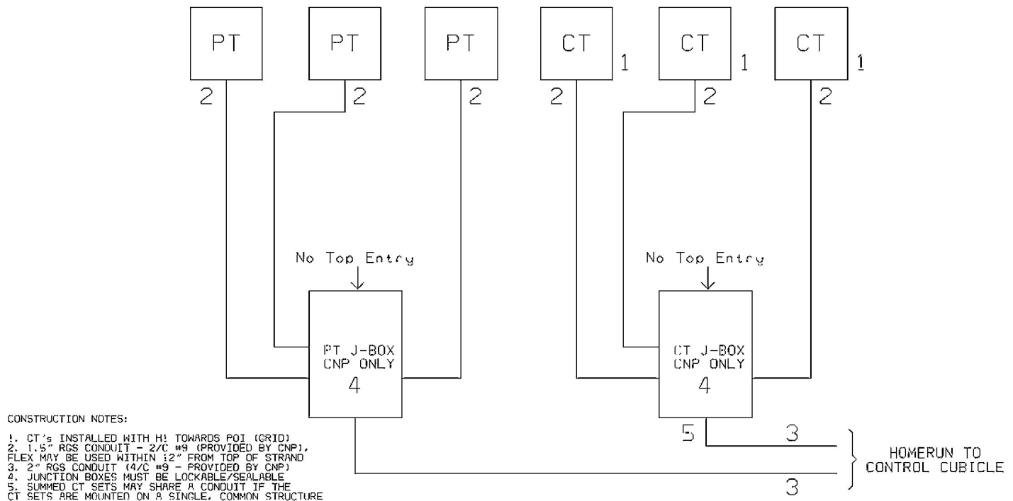
Figure 2: Junction Box Layout
