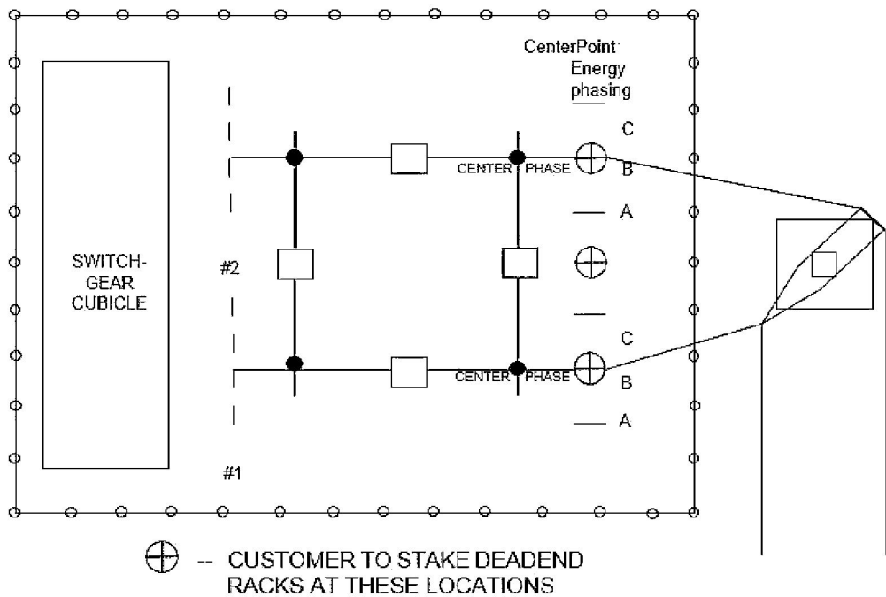
Staking Requirements for Typical Customer Substation
