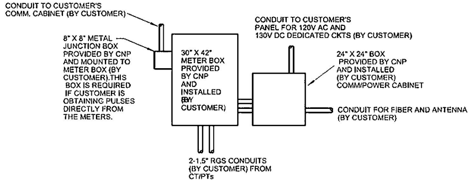
Figure 1: Control House Layout of Metering Cabinets
