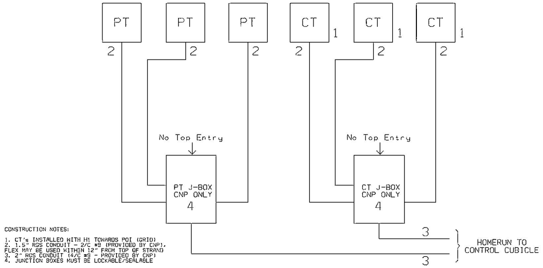
Figure 2: Junction Box Layout
