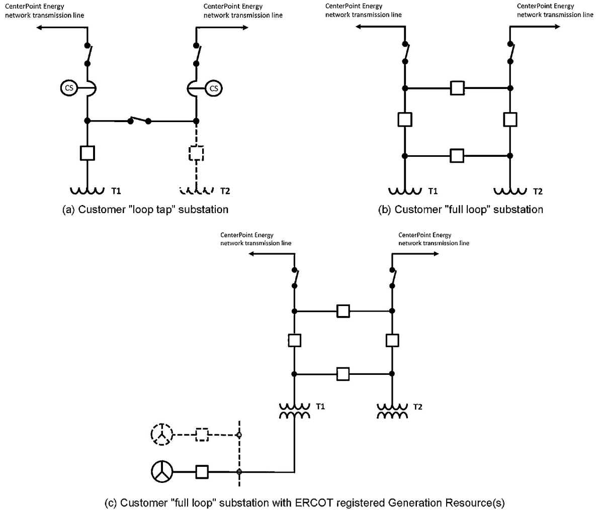
Figure 3 – Typical customer-owned load transmission substation interconnection arrangements
