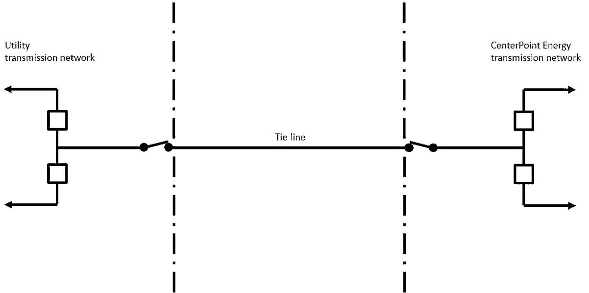
Figure 2 – Typical Utility interconnection arrangement
