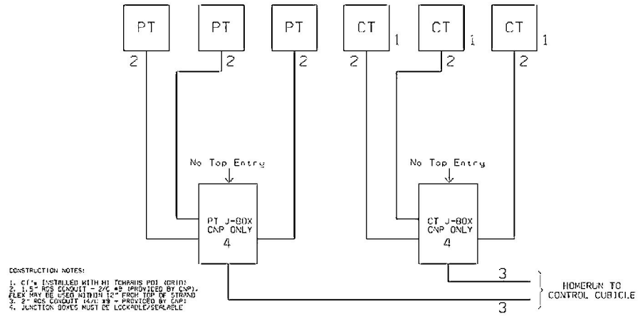
Figure 2: Junction Box Layout
