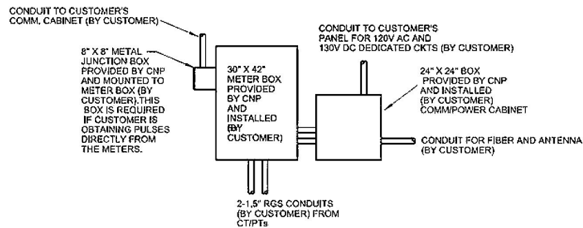
Figure 1: Control House Layout of Metering Cabinets
