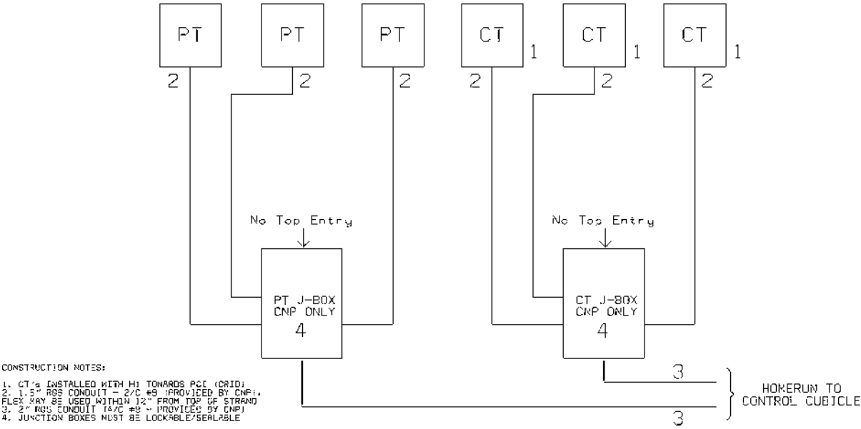
Figure 2: Junction Box Layout
