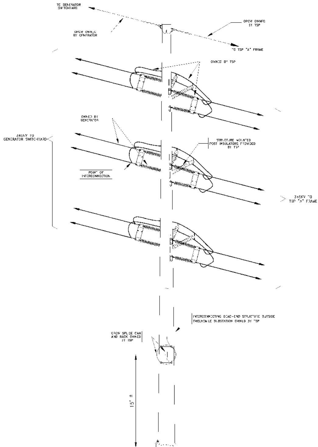
POINT OF INTERCONNECTION DETAIL
