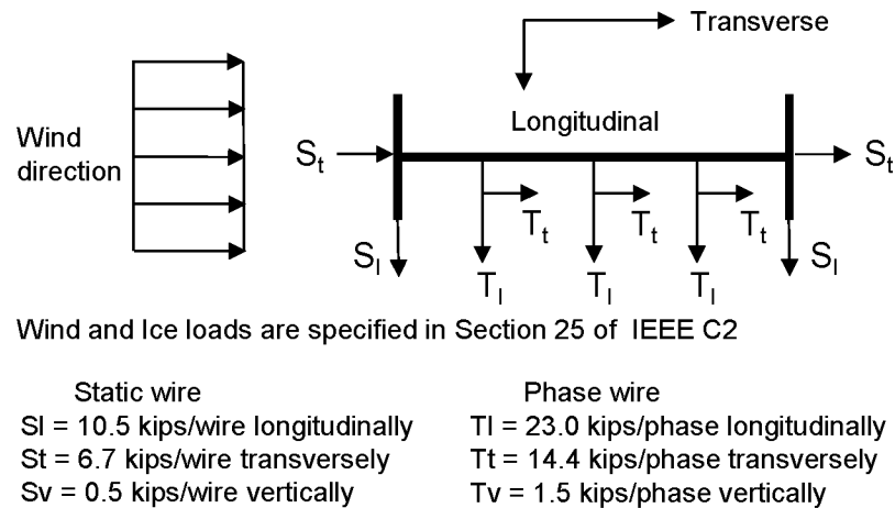
CASE 1 - Combined Ice and Wind Loading – Overhead View static wire and phase wire loading component (The static wire and phase wire loads shown include the required overload factors)
