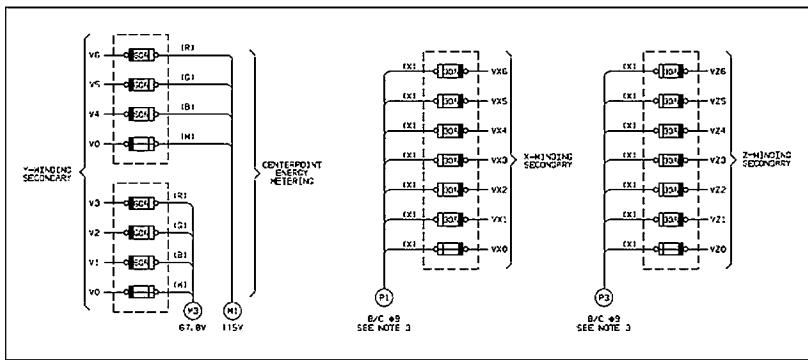
LINE #1 138KV PT PULLBOX LAYOUT
