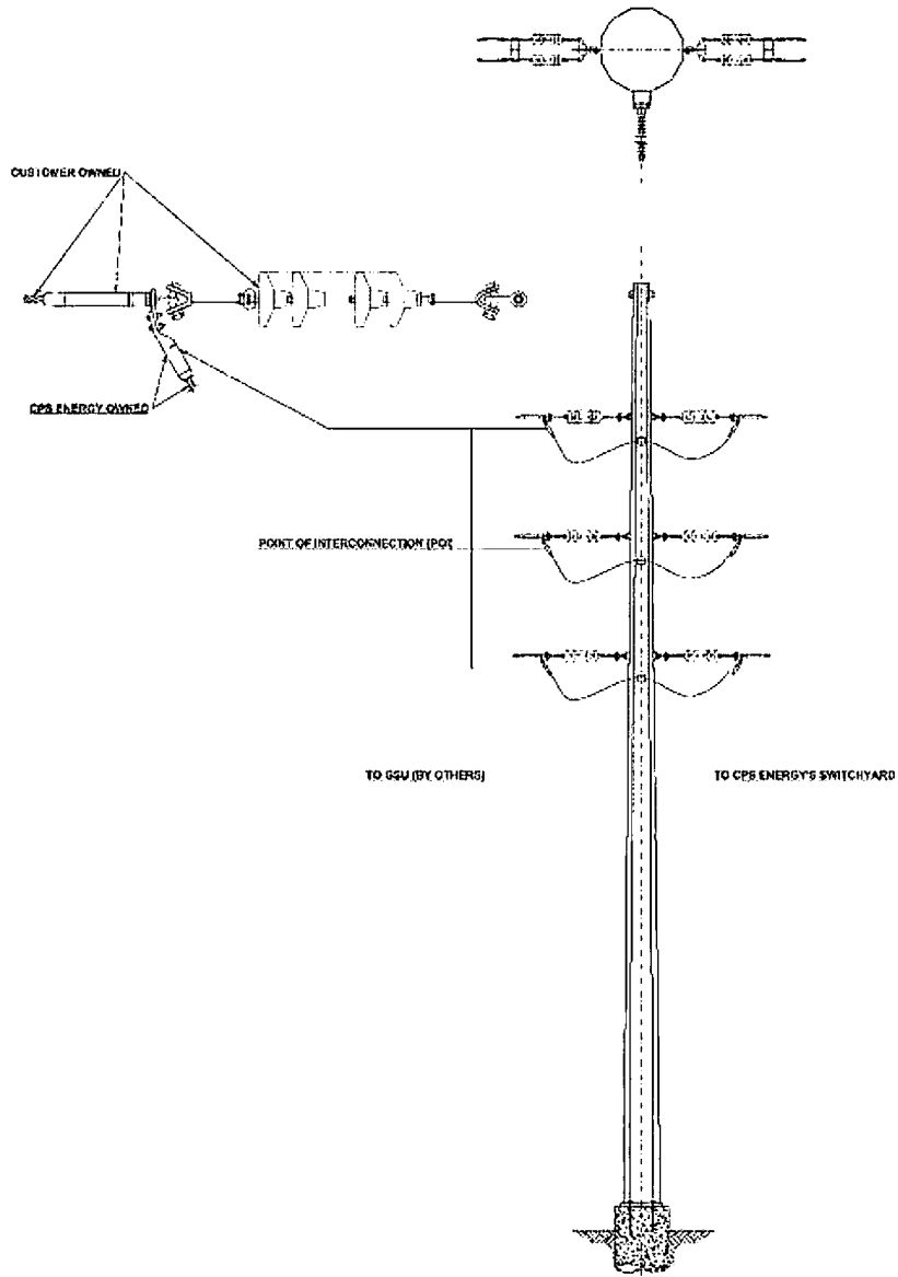
CPS Energy's last structure before Generator's facility
