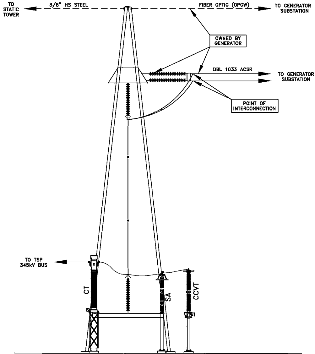
POINT OF INTERCONNECTION DETAIL
