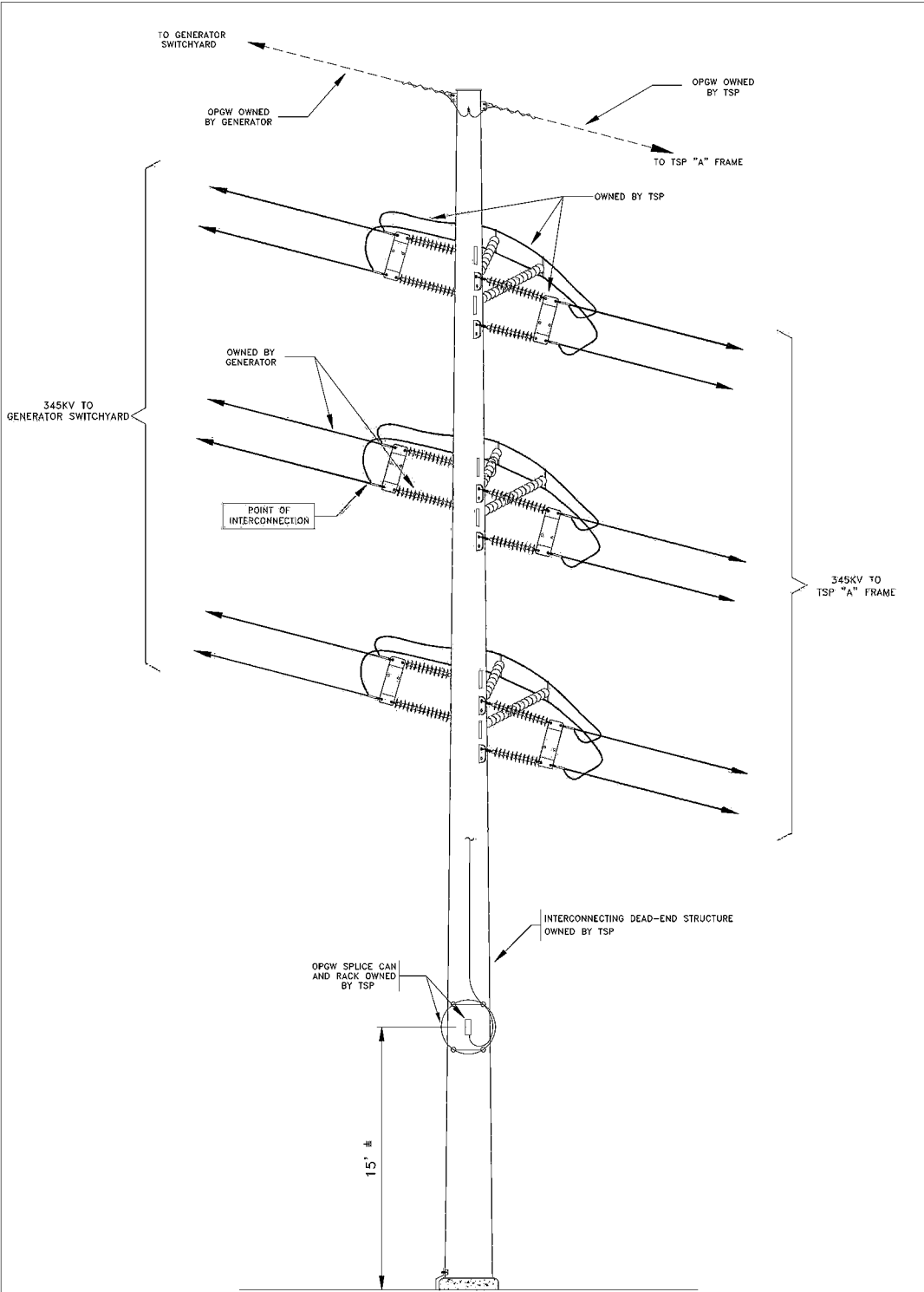
POINT OF INTERCONNECTION DETAIL
