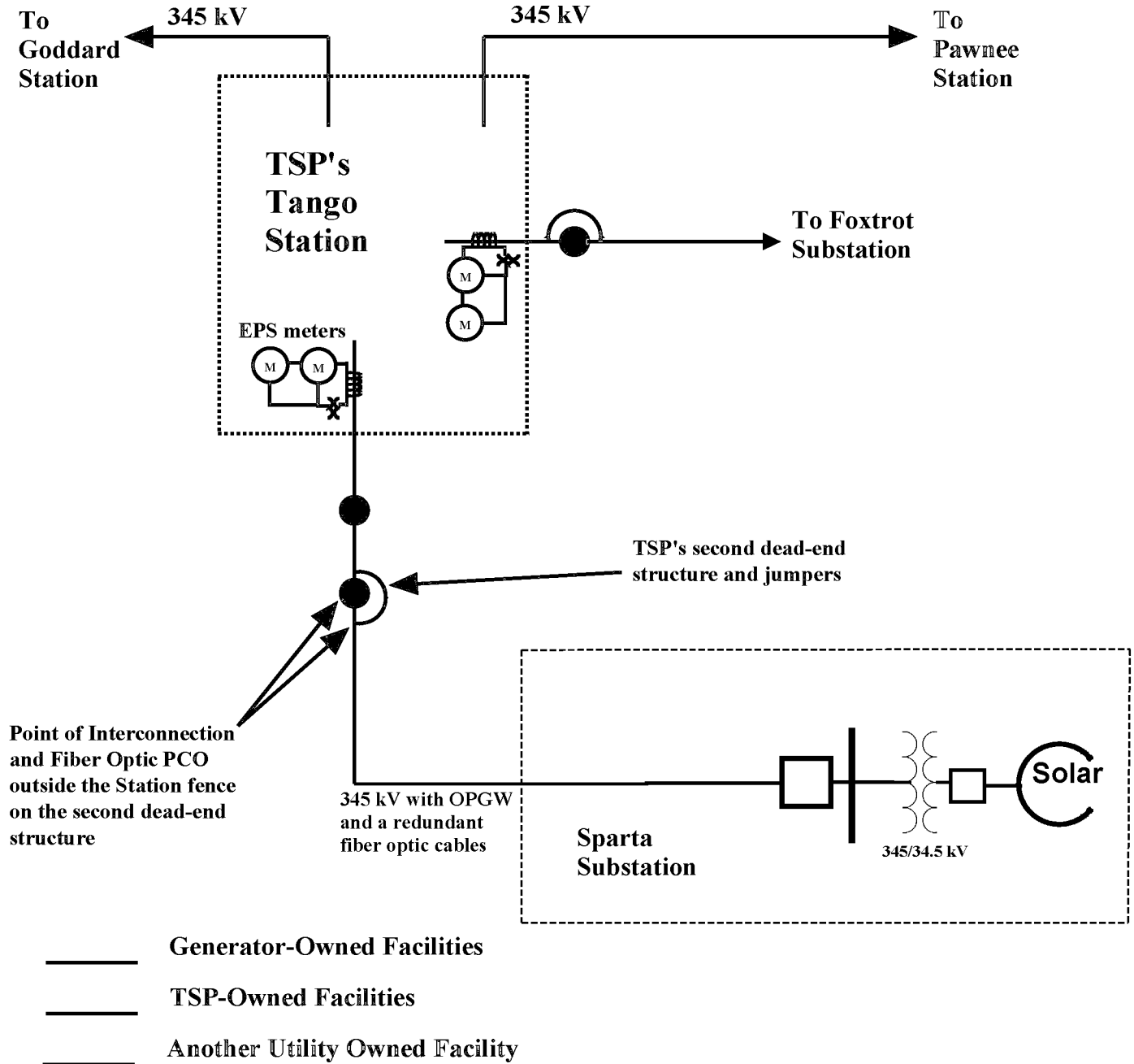
Conceptual One-Line Drawing of Point of Interconnection
