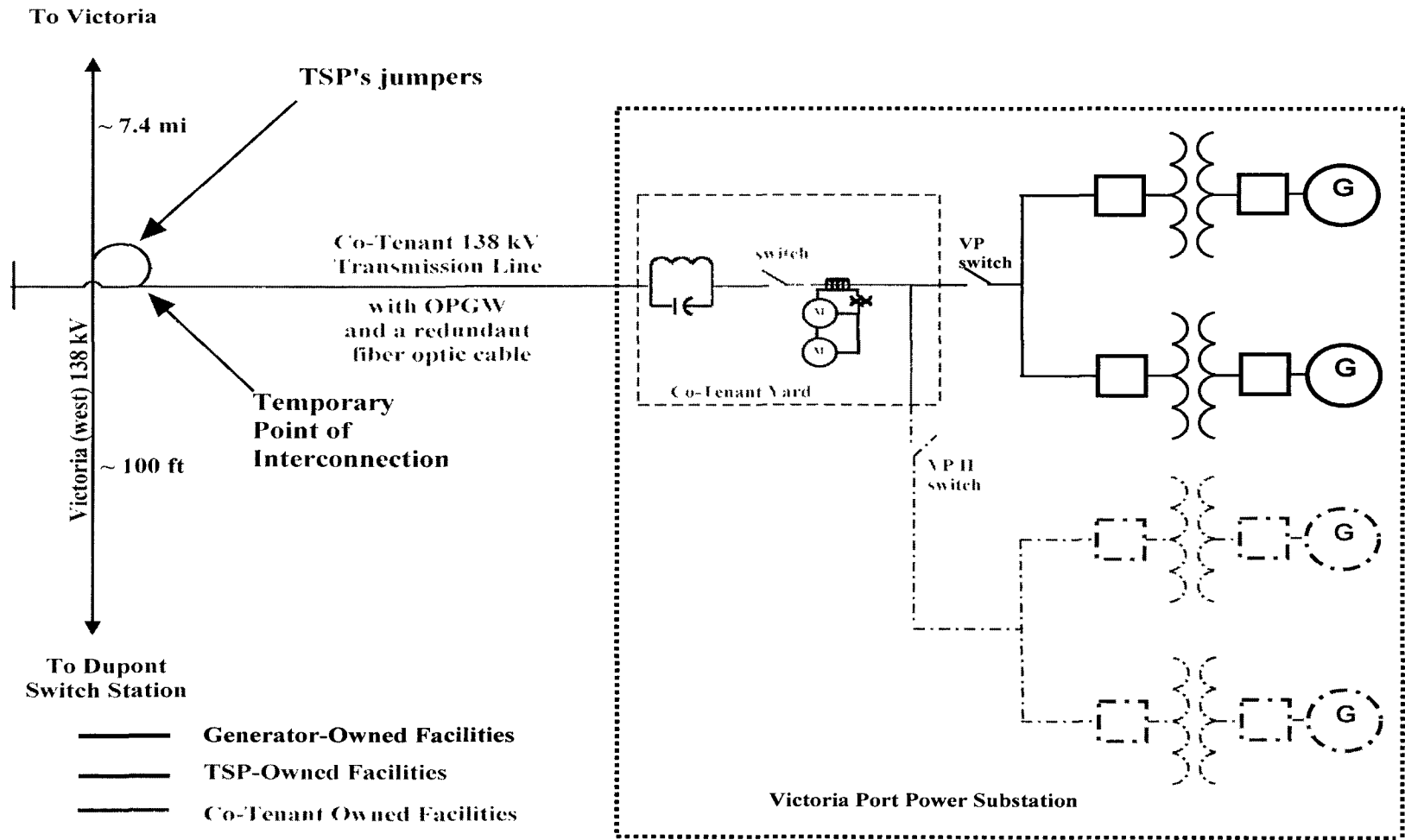
Conceptual One-Line Drawing of Temporary Facilities/Temporary Point of Interconnection
