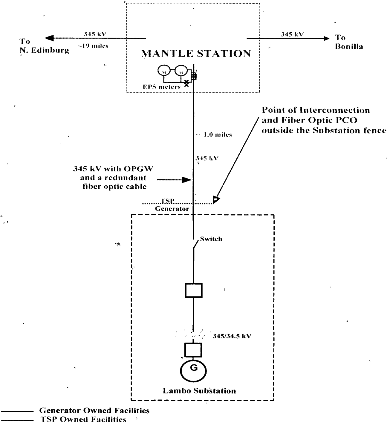
Conceptual One-Line Drawing of Point of Interconnection
