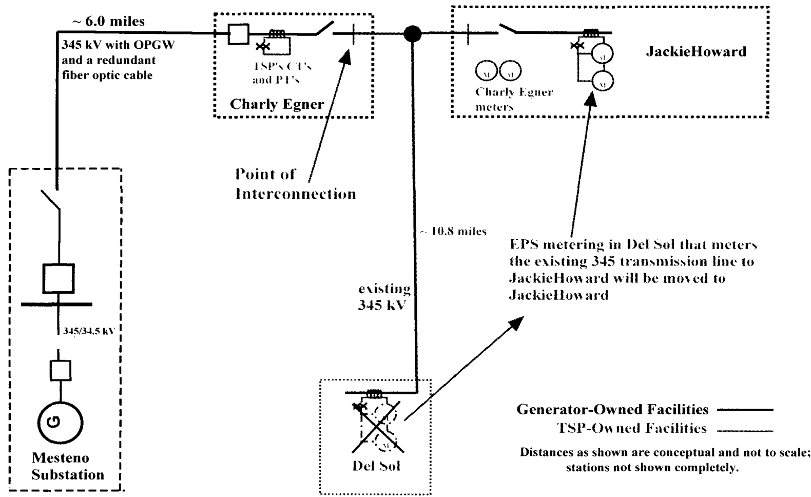
Conceptual One-Line Drawing of Point of Interconnection
