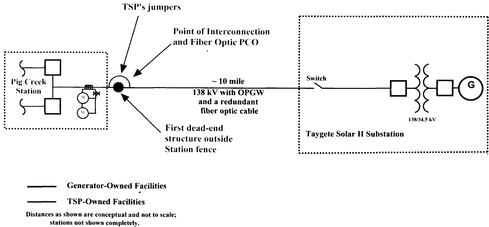
Conceptual One-Line Drawing of Point of Interconnection
