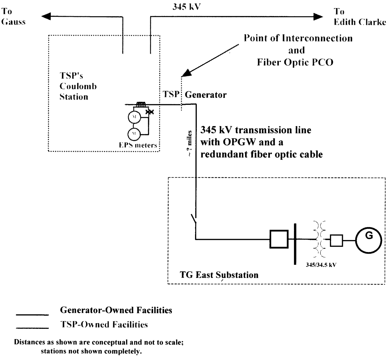
Conceptual One-Line Drawing of Point of Interconnection
