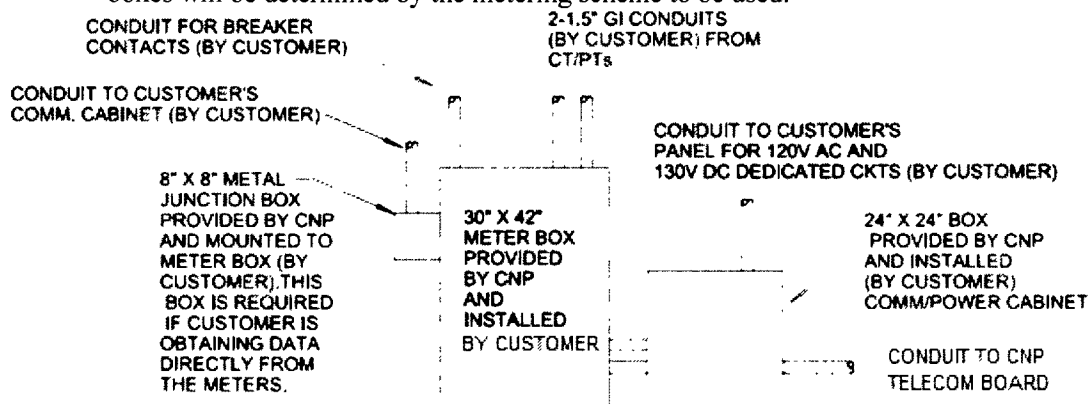
Typical Layout of Meter Boxes
