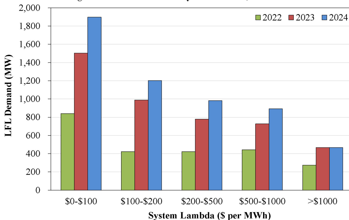
Figure 28: LFL Demand vs. System Lambda, 2022-2024
